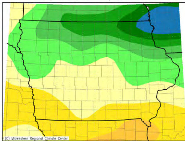
Accumulated Precipitation (in): Departure from Mean May 1, 2018 to May 31, 2018
